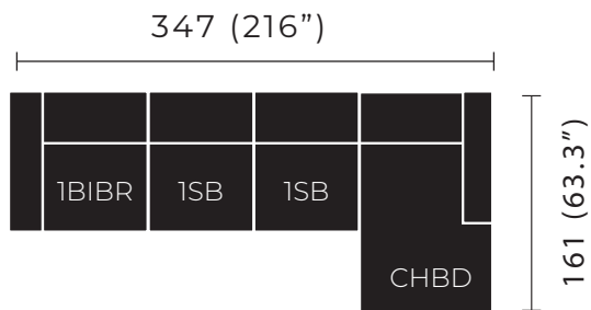
MODULAR 1B-1SB-1SB-CHB
